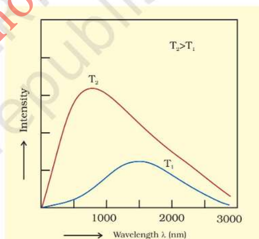
Fig. 2.8 Wavelength-intensity relationship
